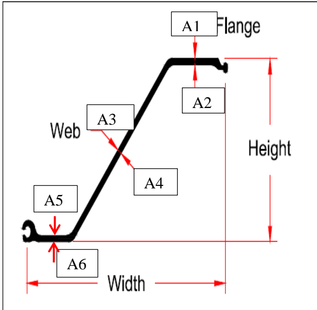
Figure 1 Sheet Piles
